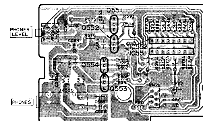
S HEADPHONES JACK P.C.B. (REP0694B)
