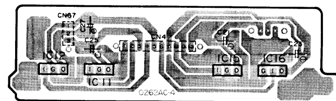
C REGULATOR IC P.C.B. (REP0693B)
