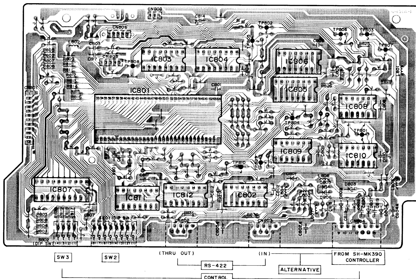
M INTERFACE P.C.B. (REP0737A)
