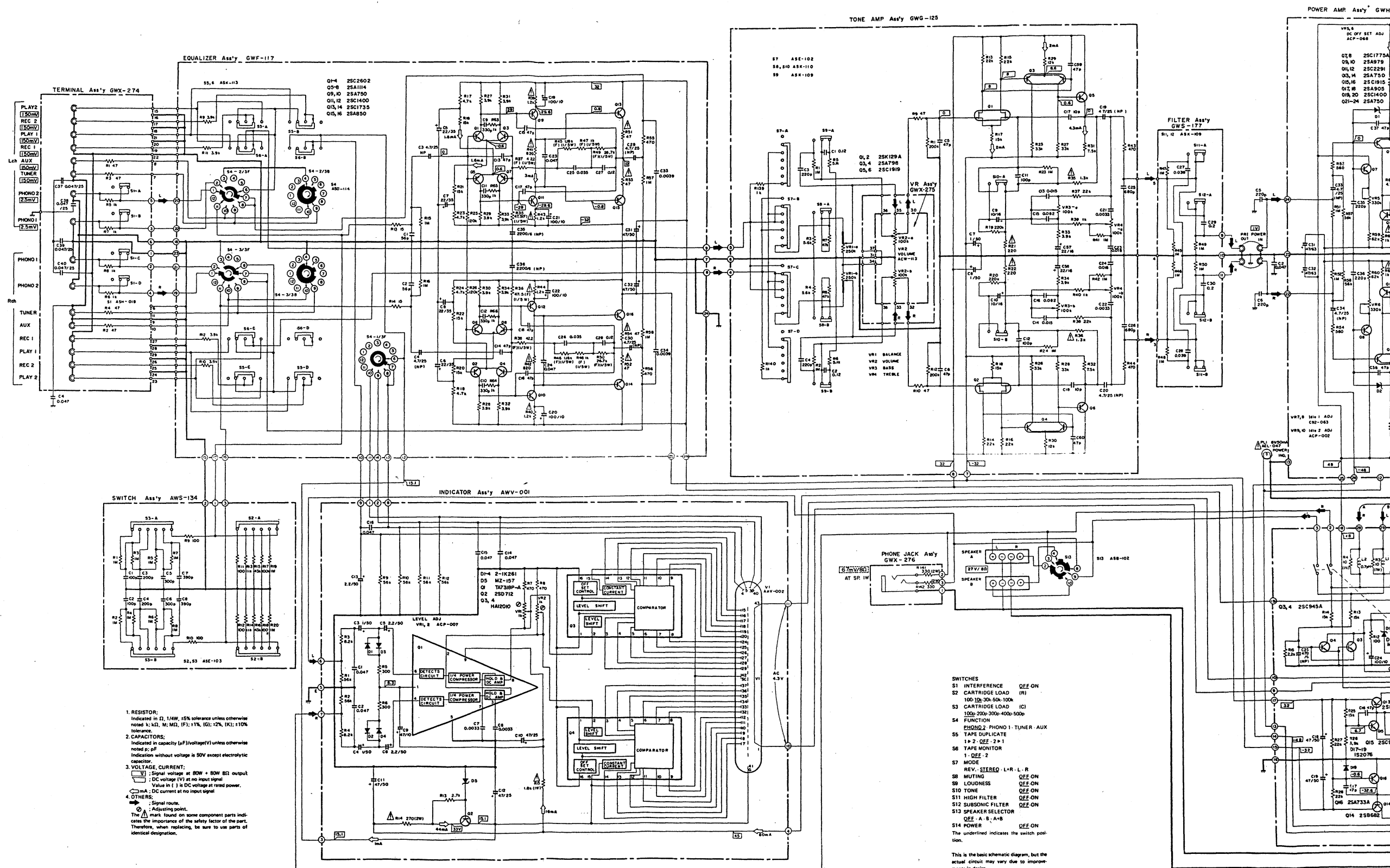
Schematic Diagram S and S/G Types
