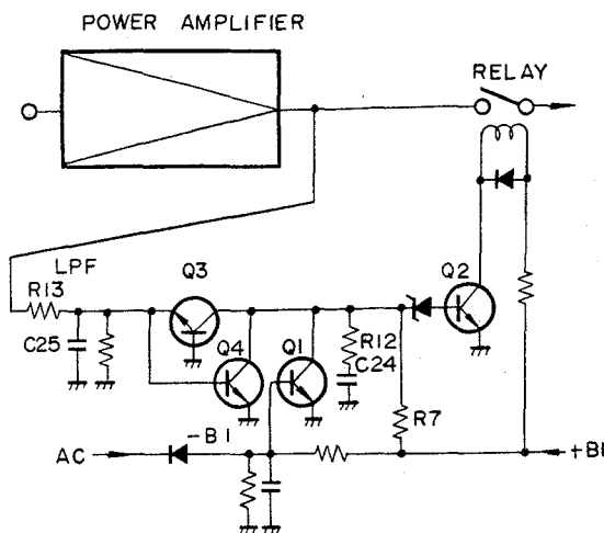
Fig. 5-11 Protection Circuit
