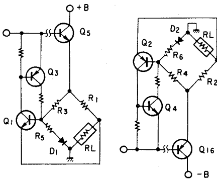
Fig. 5-5 Bridge Circuit
