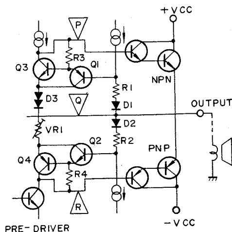
Fig. 5-7 NSA Circuit
